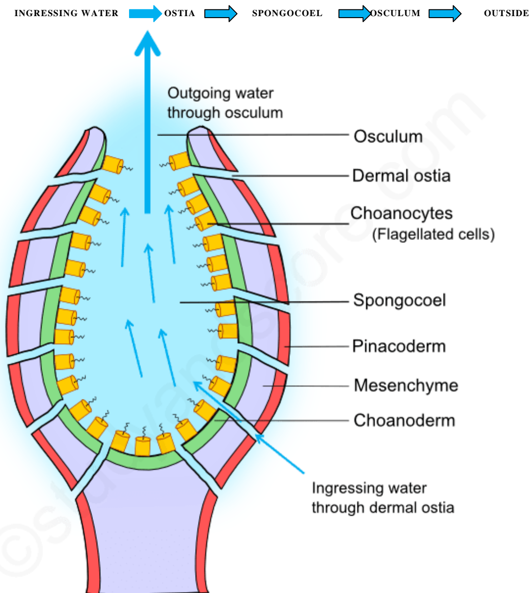
Ascon type canal system (Ex: Leucosolenia)
